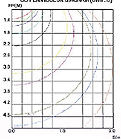
GO PLAN ISOLUX DIAGRAM (UNIT: lx)
